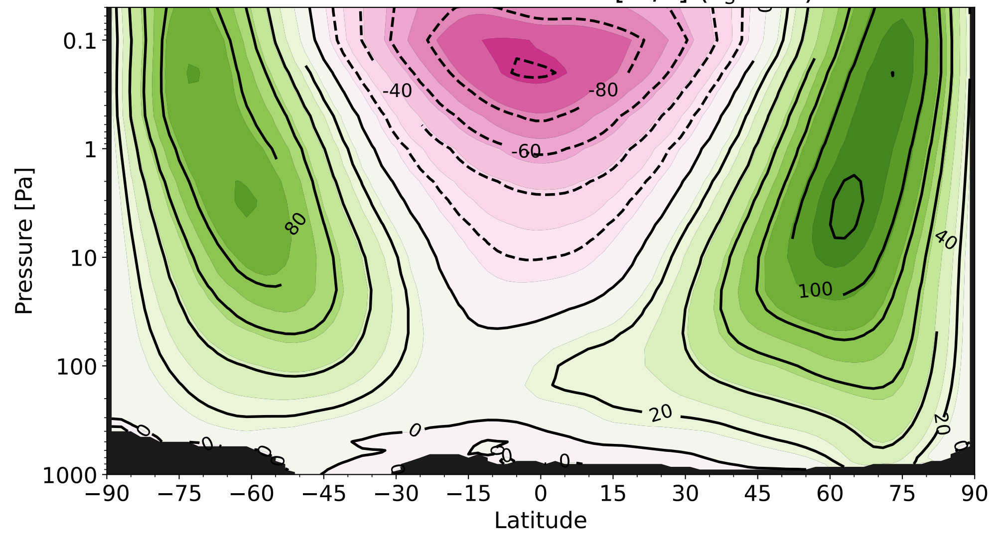
Zonal Mean Zonal Wind [m/s] ( L_s = 0^\circ )
