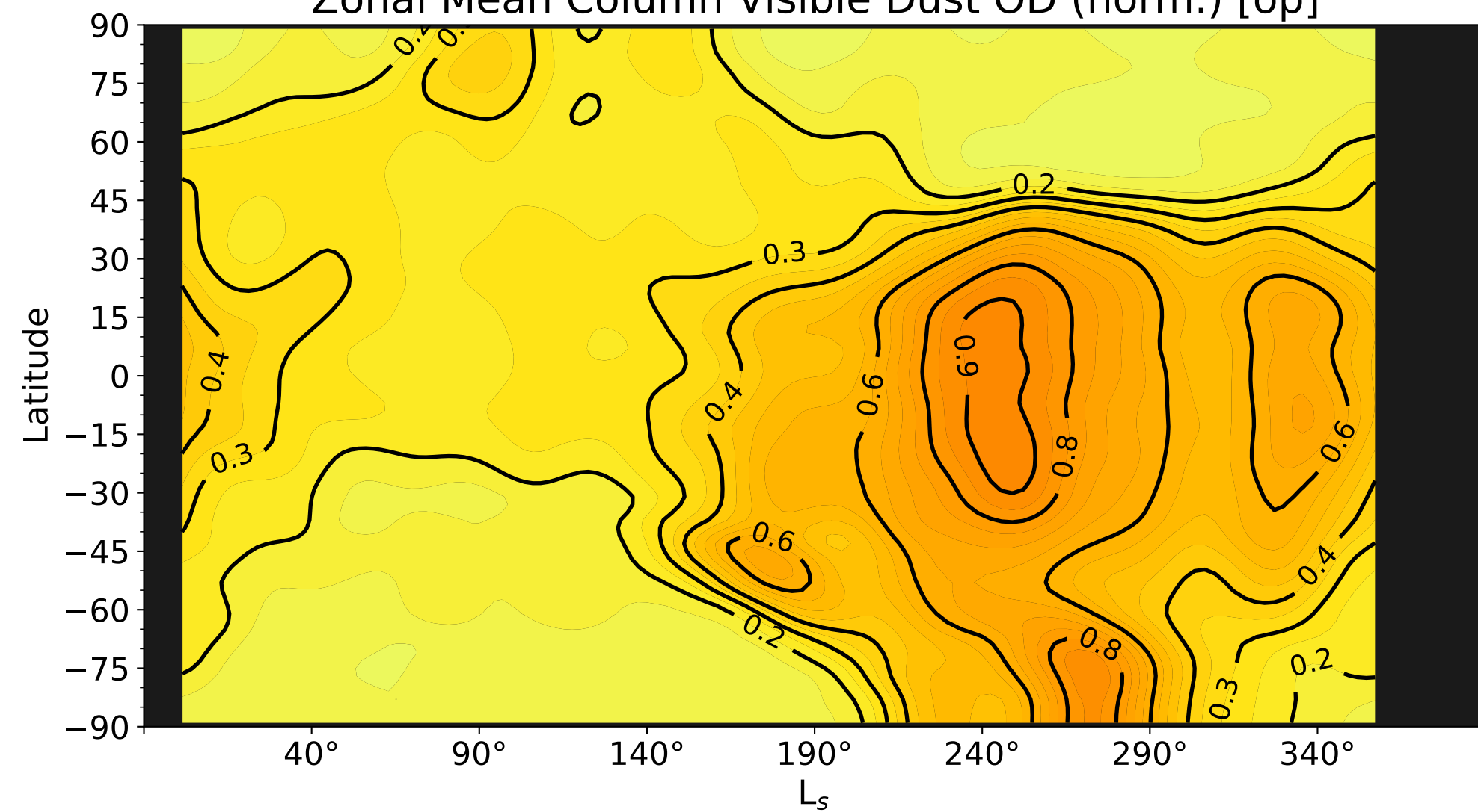
Zonal Mean Column Visible Dust OD (norm.) [op]
