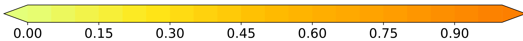
Zonal Mean Lifting Rate [ \mu\text{m/day} ]
