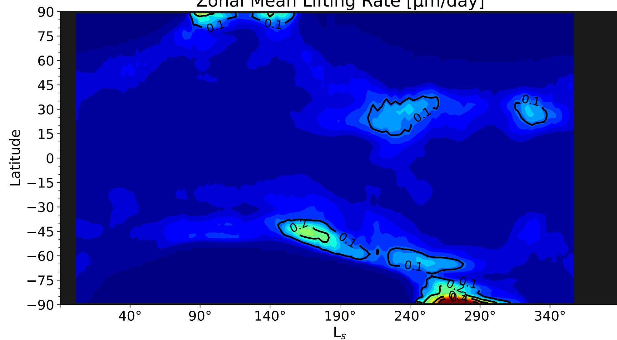
Zonal Mean Lifting Rate [ \mu\text{m/day} ]
